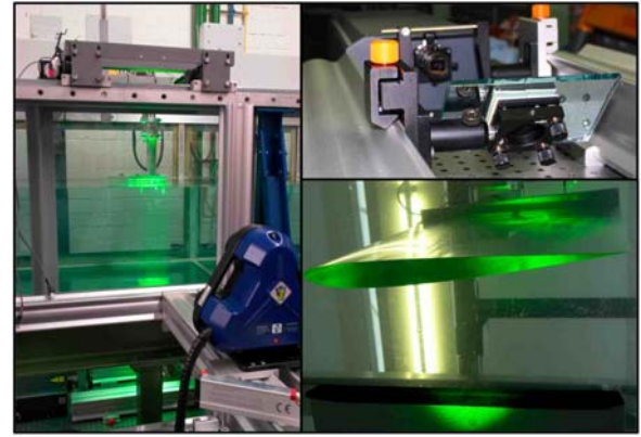
Fig. 5. Test set-up with the V3V system
