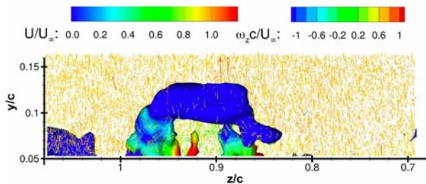
Fig. 11. Large-scale structure F; particle vectors flooded with u/u_\infty -magnitude and \lambda_2 -iso-surfaces flooded with the normalized span-wise vorticity magnitude
